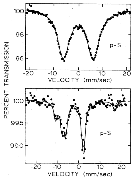
FIG. 3. Mössbauer spectra of plastic ^{125}\text{Te}_{0.01}\text{S}_{0.99} absorber (top) and plastic ^{129}\text{Te}_{0.01}\text{S}_{0.99} source (bottom) both recorded at 4.2 °K. The ^{129}\text{Te} spectrum (top) was obtained using an ^{125}\text{Sb} in Cu source. The ^{129}\text{I} spectrum (bottom) shows a fit to a pure ^{129}\text{I} quadrupole interaction with constraints on line intensities and positions. See Sec. II of text for details.
