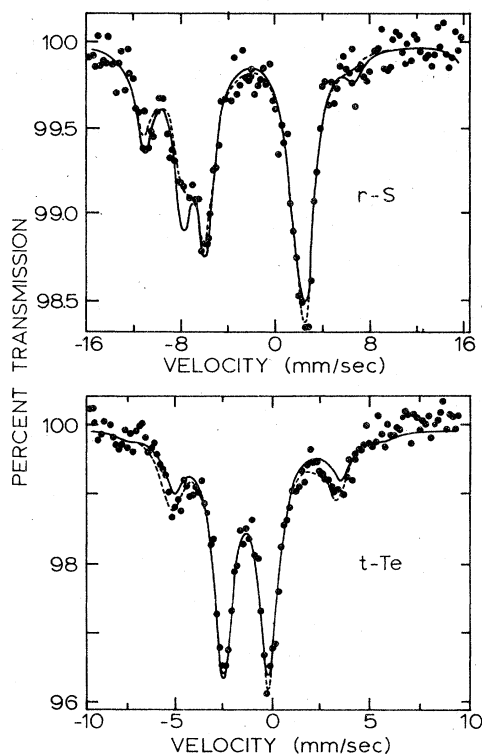
FIG. 2. Mössbauer spectra of orthorhombic ^{129}\text{Te}_{0.01}^m\text{S}_{0.99} ( r -S) and trigonal ^{129}\text{Te}^m ( t -Te) sources recorded at 4.2 °K. The continuous-line fit represents an analysis of these spectra to a pure ^{129}\text{I} quadrupole interaction with the line intensities and positions constrained. See Sec. II of text for details. The broken line fit is obtained when constraints on line intensities are lifted.
