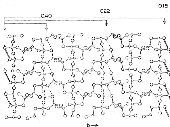
FIG. 8. Fragment of the high-temperature phase of c - \text{GeSe}_2 showing corner-sharing chains running laterally along the b axis. The small circles represent fourfold coordinated Ge atoms, while the larger circles represent twofold-coordinated Se atoms. In the glass this fragment is believed to be bordered by Se-Se dimers. This fragment, also known as a "raft," is thus Se-rich. The degree of broken chemical order (DBO) of the glass network is "raft"-size dependent. In particular, for a two-chain "raft" the DBO is 0.4, while for a six-chain "raft" the DBO is 0.15. The observed DBO in \text{GeSe}_2 glass is compatible with a six-chain "raft," i.e., a cluster about 50 Å wide.
