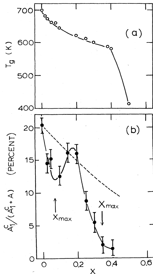
FIG. 1. (a) Glass transitions ( T_g ) of \text{Ge}_{1-x}\text{Sn}_x\text{Se}_2 glasses plotted as a function of x . (b) Normalized A_1^c / (A_1^c + A) scattering strength of the A_1^c - \text{Ge}(\text{Se}_{1/2})_4 companion mode in Raman spectra of \text{Ge}_{1-x}\text{Sn}_x\text{Se}_2 glasses plotted as a function of x . Here, A represents the sum of the A_1 - \text{Ge}(\text{Se}_{1/2})_4 , A_1 - \text{Sn}(\text{Se}_{1/2})_4 , and A_1^c - \text{Sn}(\text{Se}_{1/2})_4 mode strengths. The dashed line is the expected x variation of the A_1^c -mode strength in a model where Sn randomly replaces Ge in the \text{GeSe}_2 network. The observed extinction of the A_1^c mode near x=0.40 indicates that a structural transition occurs in these glasses between x=0.20 and 0.40 . The secondary maximum near x=0.20 may arise from an intermediate stage in cluster degradation, where the six-chain "rafts" present at x=0 are replaced by two-chain "rafts." See Fig. 8 for details.
