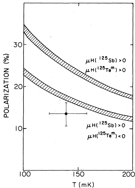
FIG. 4. Calculated and observed polarization in the NOME spectrum of ^{125}\text{Te} in \text{Pd}_2\text{MnSb} .
